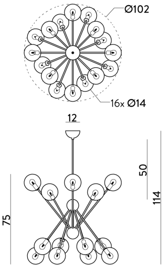
Product Dimensions
