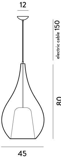
Product Dimensions
