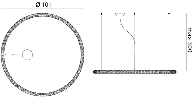
Product Dimensions
