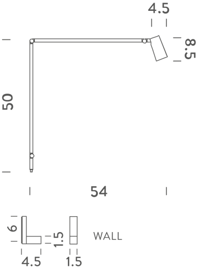
Product Dimensions
