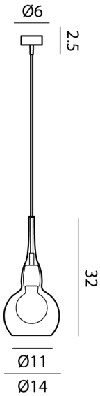
Product Dimensions
