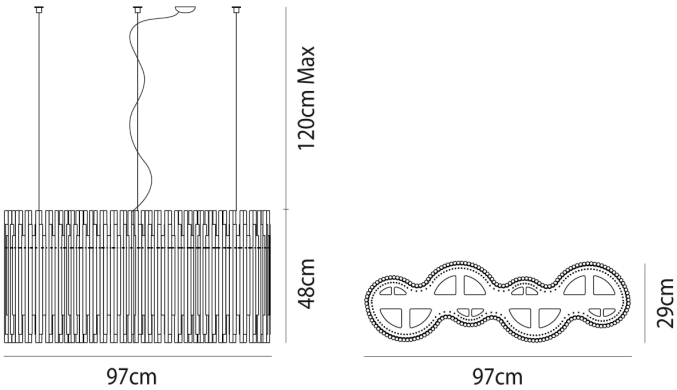
Product Dimensions
