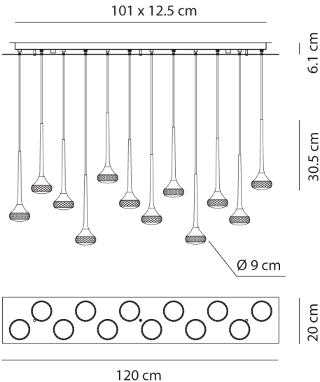
Product Dimensions
