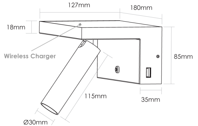
Product Dimensions
