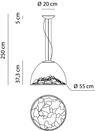
Product Dimensions
