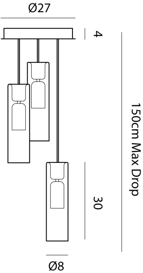
Product Dimensions
