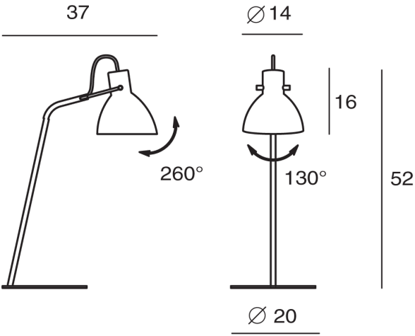
Product Dimensions
