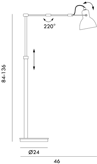
Product Dimensions
