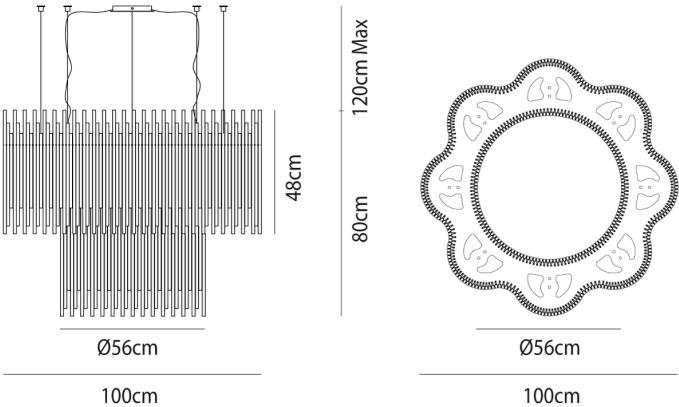
Product Dimensions
