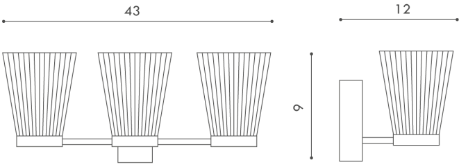
Product Dimensions
