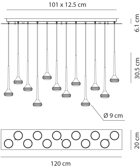
Product Dimensions
