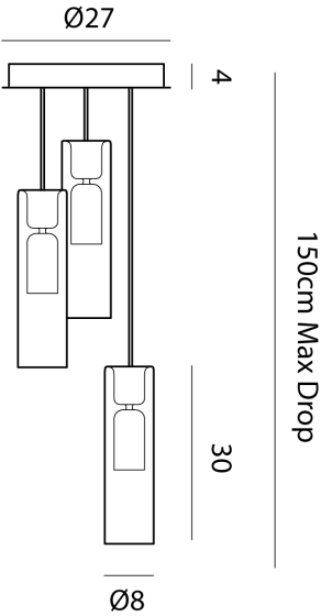
Product Dimensions
