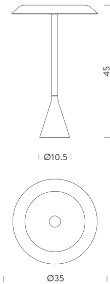
Product Dimensions
