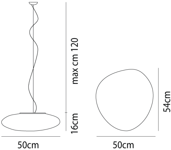
Product Dimensions
