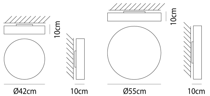
Product Dimensions
