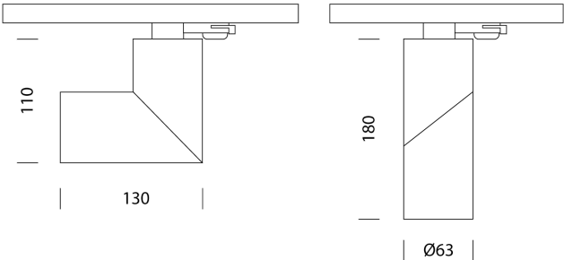
Product Dimensions
