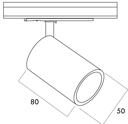
Product Dimensions
