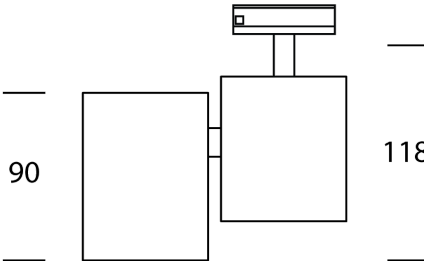
Product Dimensions
