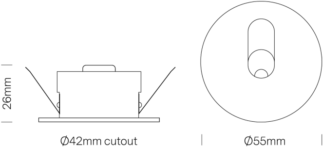
Product Dimensions
