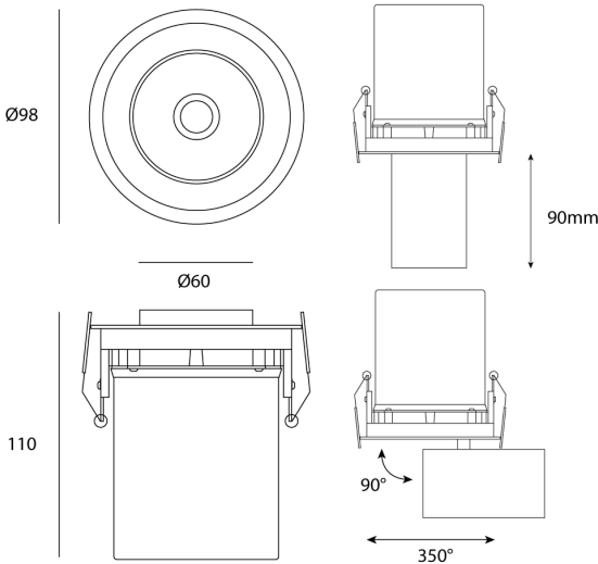
Product Dimensions
