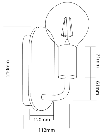
Product Dimensions
