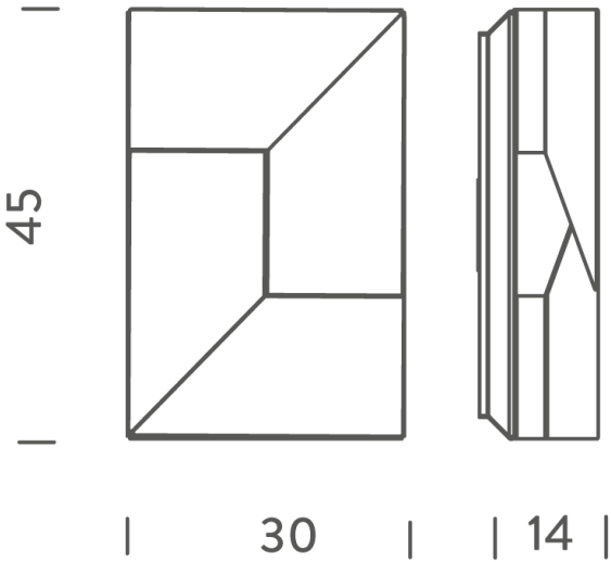
Product Dimensions
