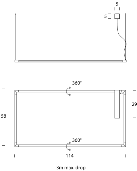
Product Dimensions
