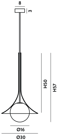
Product Dimensions
