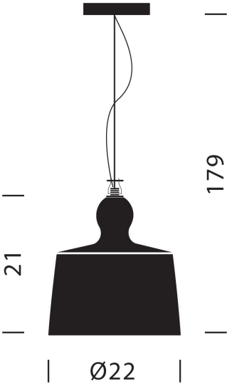
Product Dimensions
