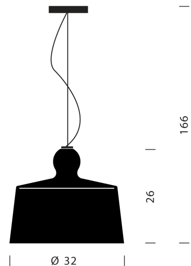
Product Dimensions
