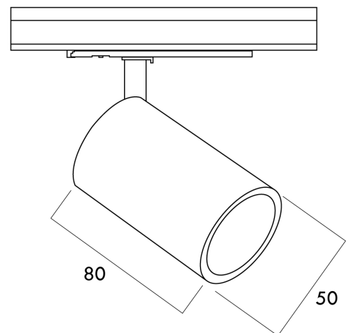
Product Dimensions
