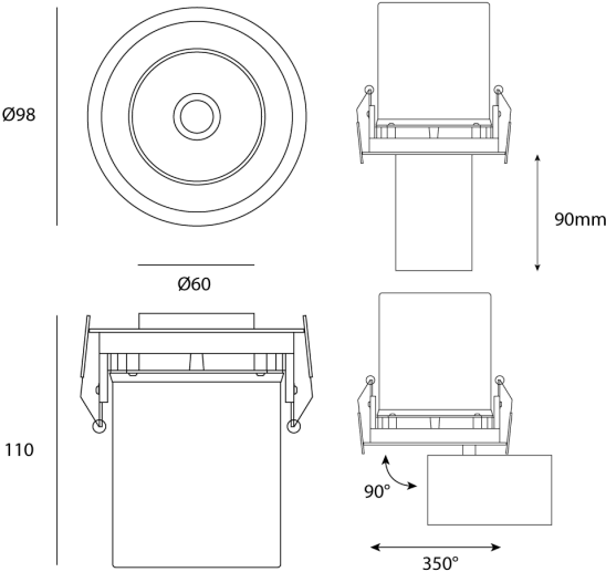
Product Dimensions
