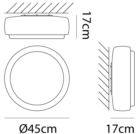
Product Dimensions
