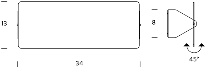
Product Dimensions
