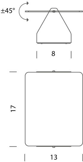
Product Dimensions
