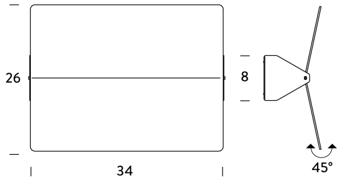
Product Dimensions
