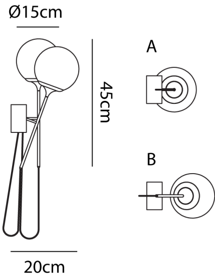
Product Dimensions
