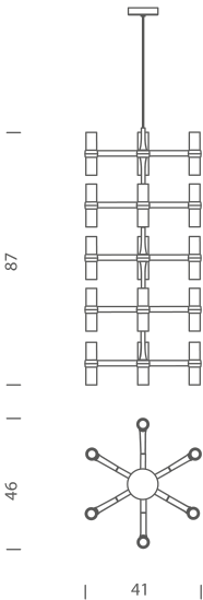
Product Dimensions
