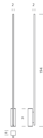
Product Dimensions
