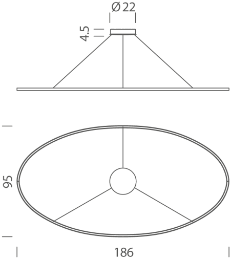
Product Dimensions
