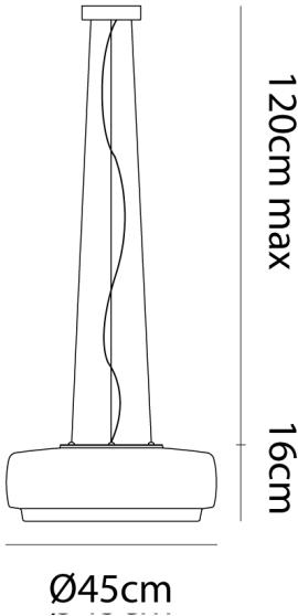
Product Dimensions
