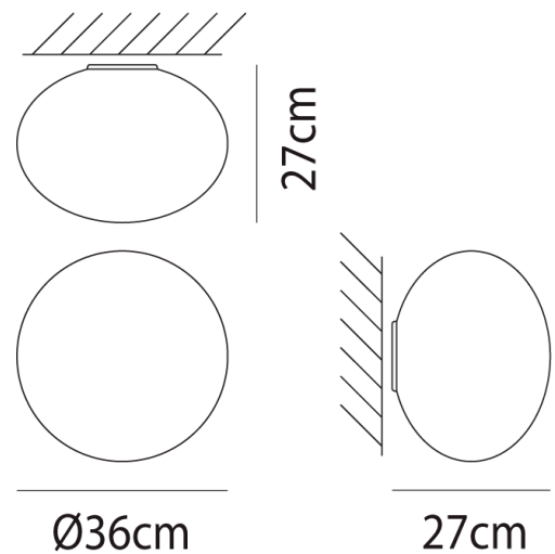
Product Dimensions
