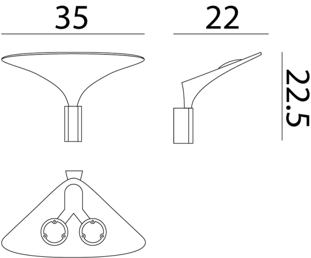
Product Dimensions
