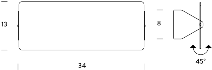
Product Dimensions
