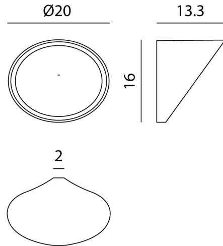
Product Dimensions
