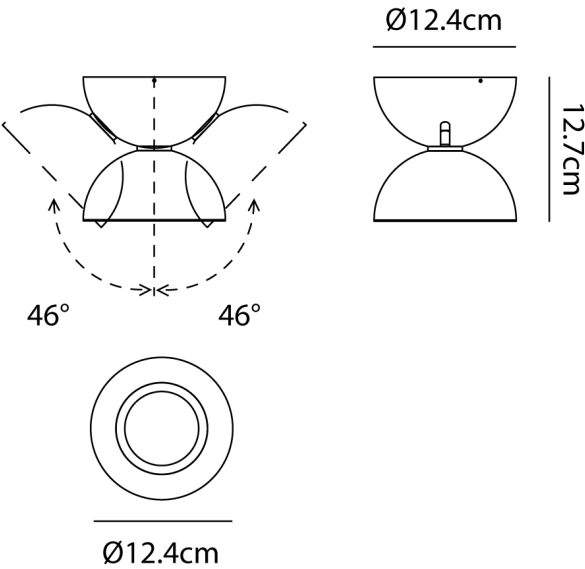
Product Dimensions
