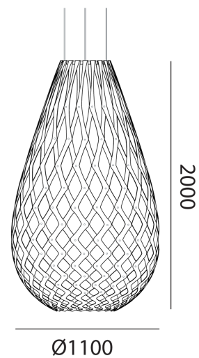
Product Dimensions
