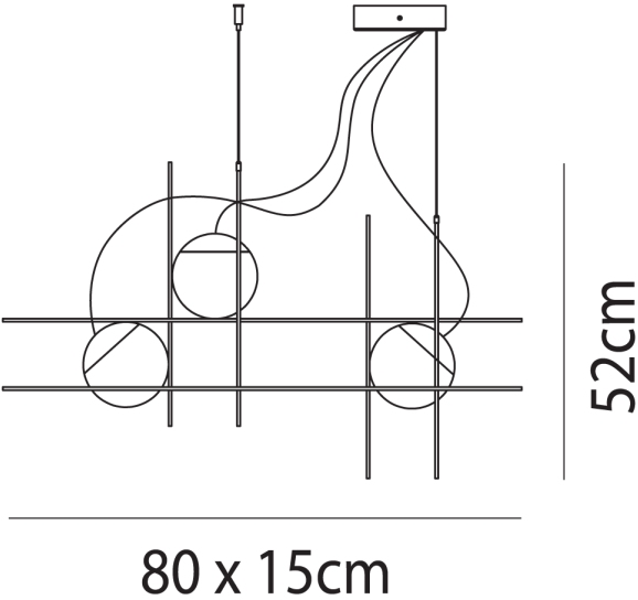
Product Dimensions
