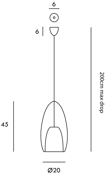
Product Dimensions
