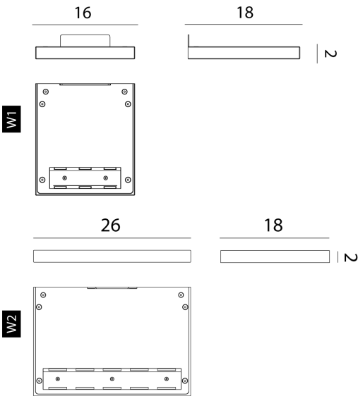
Product Dimensions
